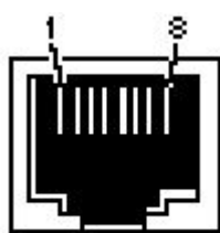
RJ-45 port
